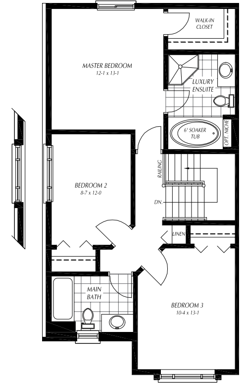
SECOND FLOOR PLAN OPTION 3
