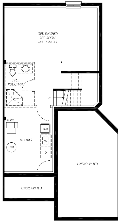
BASEMENT PLAN
